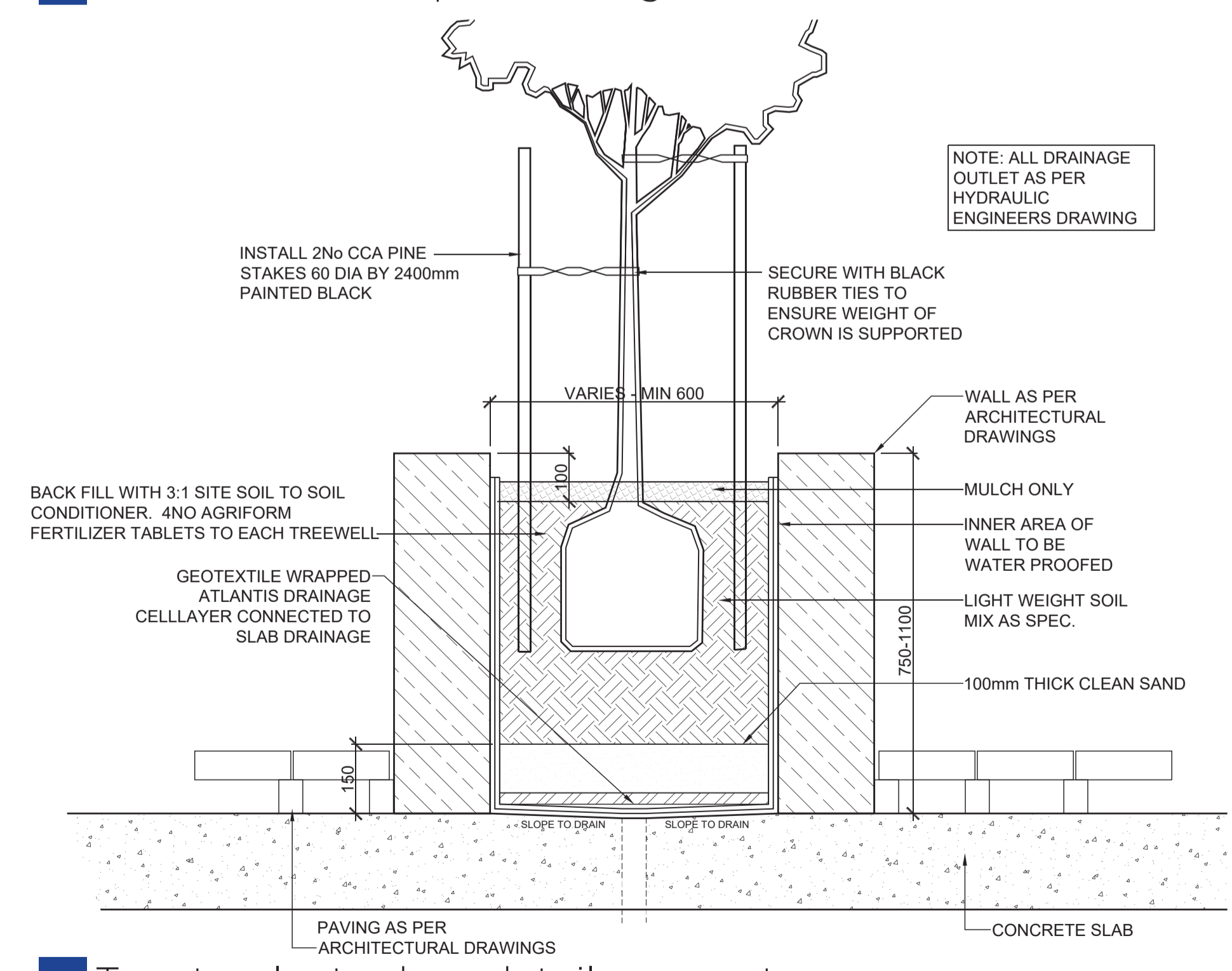
Tree to planter box detail nts
